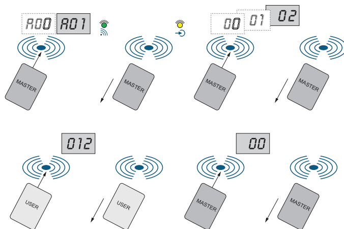
Example 2: how to code the card with number 12 to activate relay 2 only.
