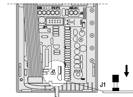
Cable art. SMT130
